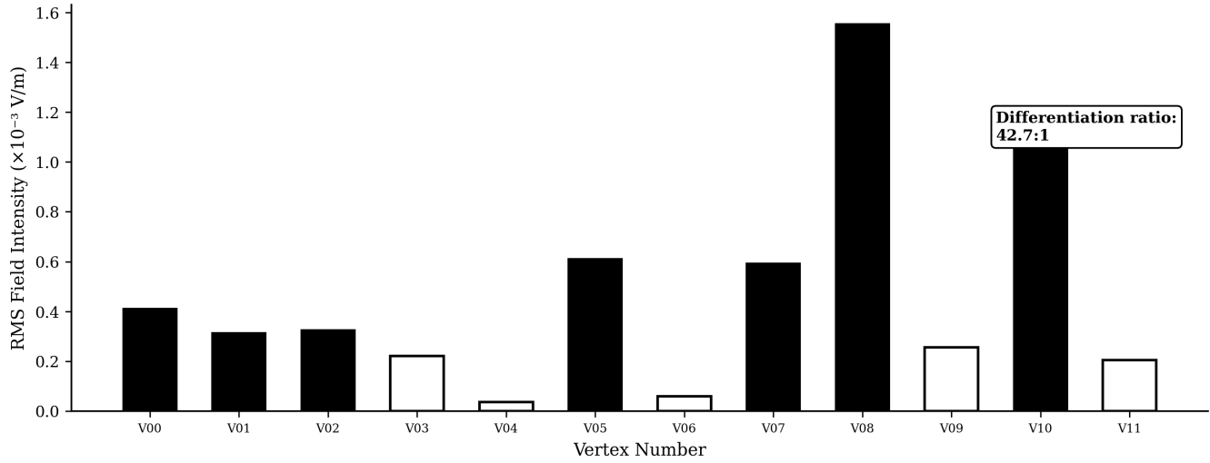
Vertex Field Intensity at 1.5 GHz (Fundamental)
