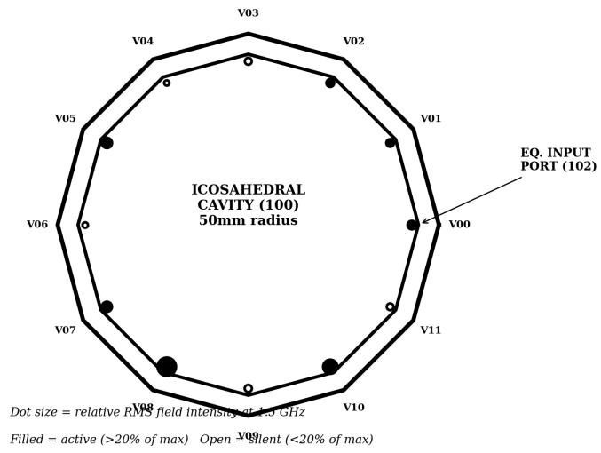
Vertex Field Intensity at 1.5 GHz (Fundamental)
